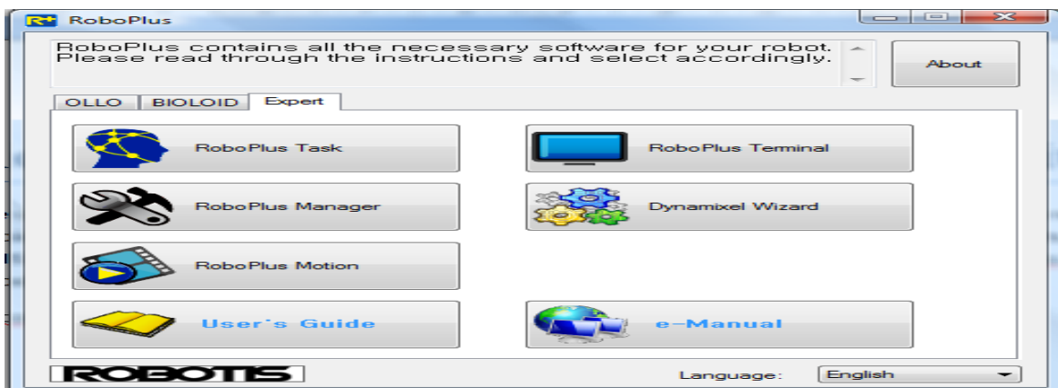
Figura 5.2 Software RoboPlus
